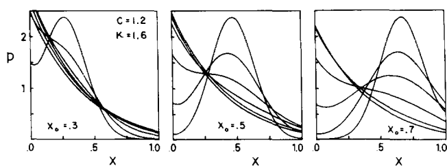
FIG. 5. The solution for the probability distribution p(x,t|x_0) [Eq. (41)] for one combination of c and \kappa , and different initial distributions (different x_0 ). The time evolution of p , from an initial \delta function to a final exponential with time-decreasing normalization constant, is shown for (in order of decreasing amplitude at x_0 ) t = 0.01, 0.02, 0.04, 0.08, 0.16, 0.32 . In this work x_N = D = 1 .
