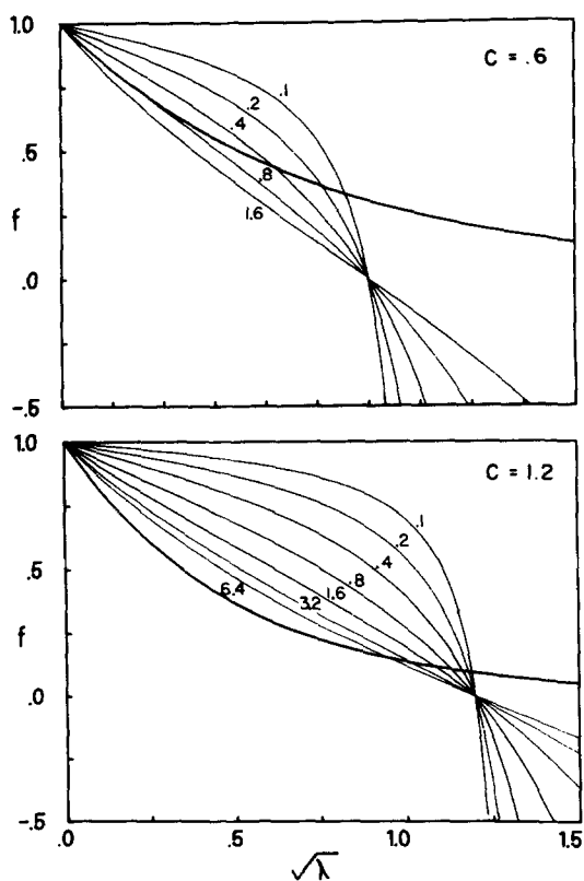
FIG. 2. Graphical solution for \lambda_0 from Eq. (33). The thick line is f_r , and the thin lines are f_l for the designated values of \kappa . In this work x_N = 1 and D = 1 .
