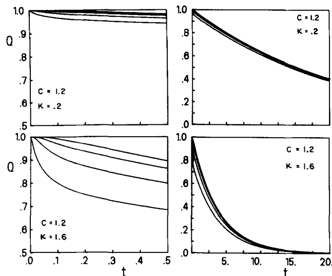
FIG. 7. Same as Fig. 6 for c = 1.2 .
