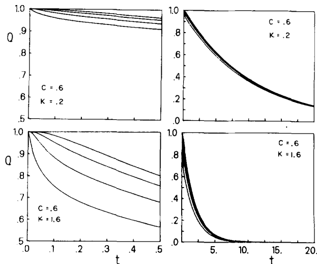
FIG. 6. The solution for the survival probability Q(t|x_0) [Eq. (42)] for c = 0.6 and two values of \kappa . The four lines are for (top to bottom) x_0 = 0.3, 0.5, 0.7 , and 0.9 . The left panels demonstrate short time behavior, whereas the right panels show the long time behavior. In this work x_N = 1 and D = 1 .
